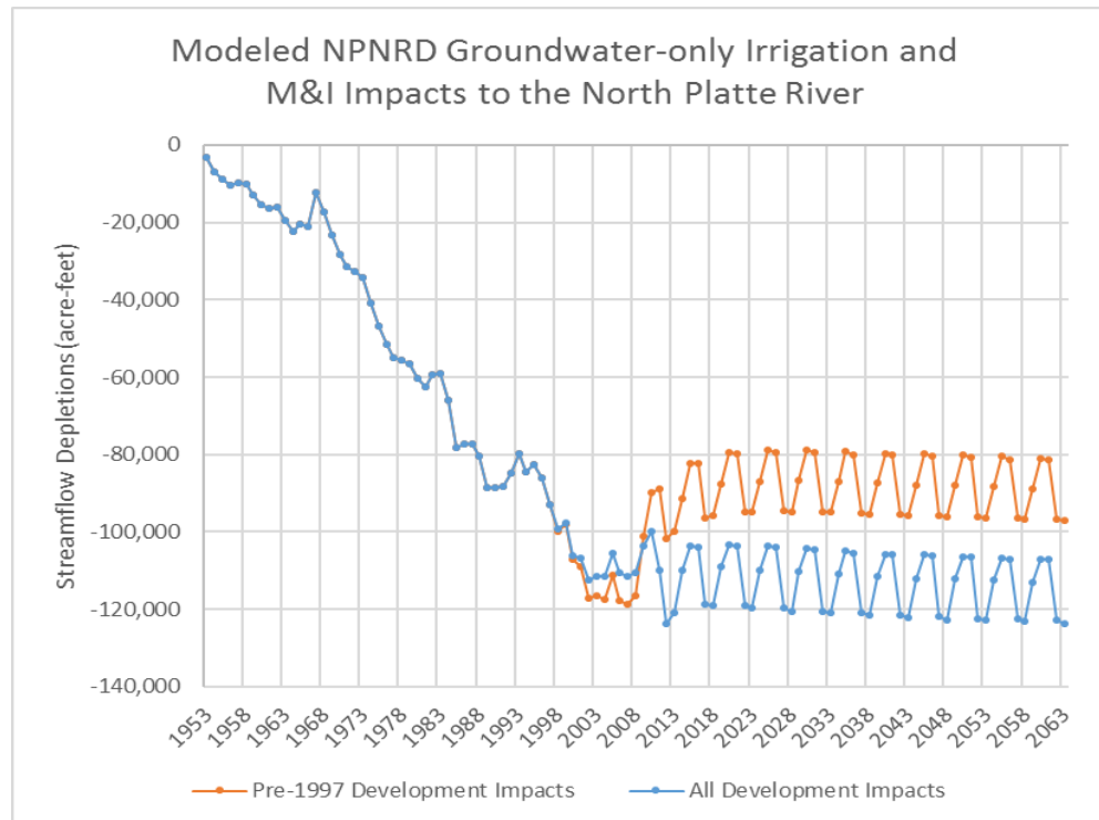
Figure 6. Modeled NPNRD streamflow impacts to the North Platte River from all groundwater-only irrigation and municipal and industrial (M&I) development with offsetting management actions and the streamflow impacts from development pre-1997
