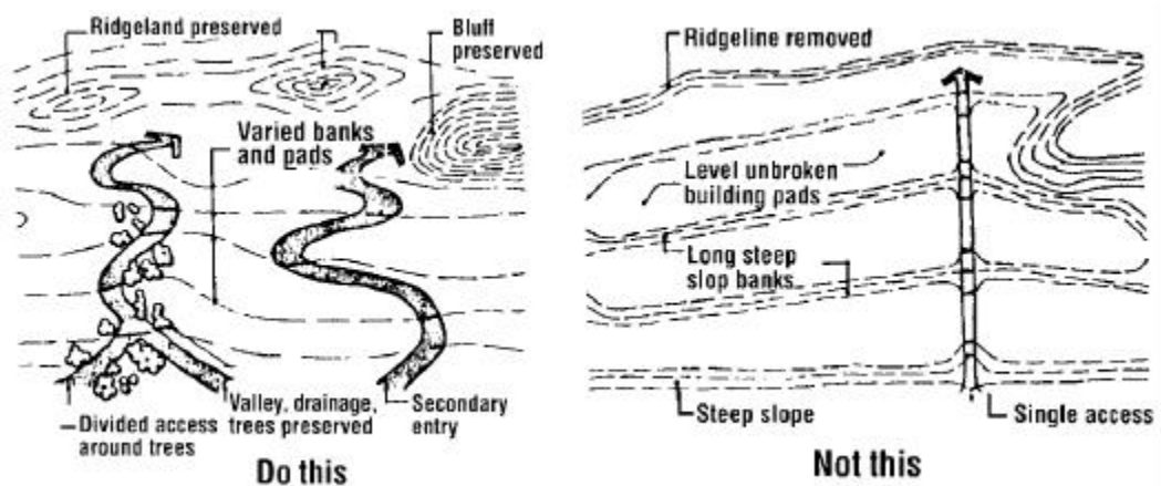
Figure 6-5. Los Angeles County's hillside grading guidelines.
