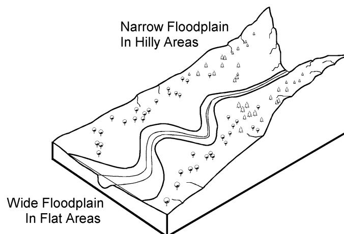
Figure 1-3. Riverine floodplain
