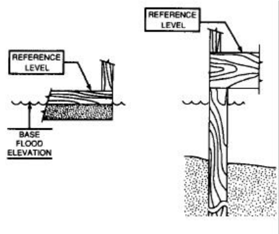
Figure 5-11. In A Zones: the top of the floor is the reference level
