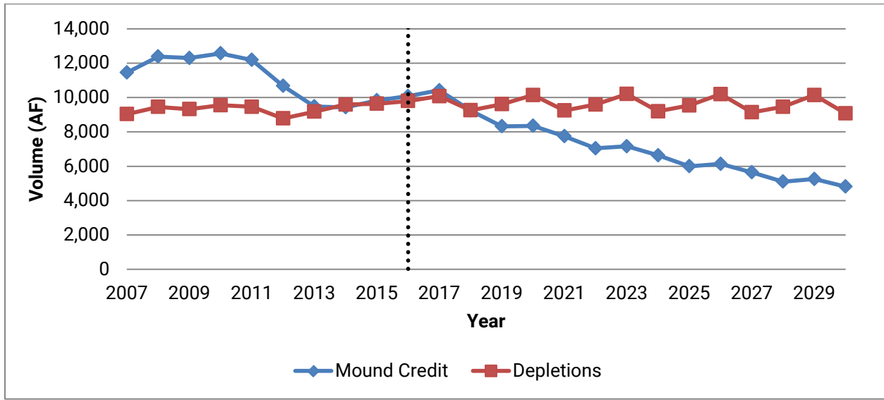
Figure A. 3-Year Mound Credit and Groundwater Depletions (AF) at the TBNRD Southern Boundary. Data from 2011-2013 were projected forward from 2016 to represent a potential outcome under a dryer climate cycle.
