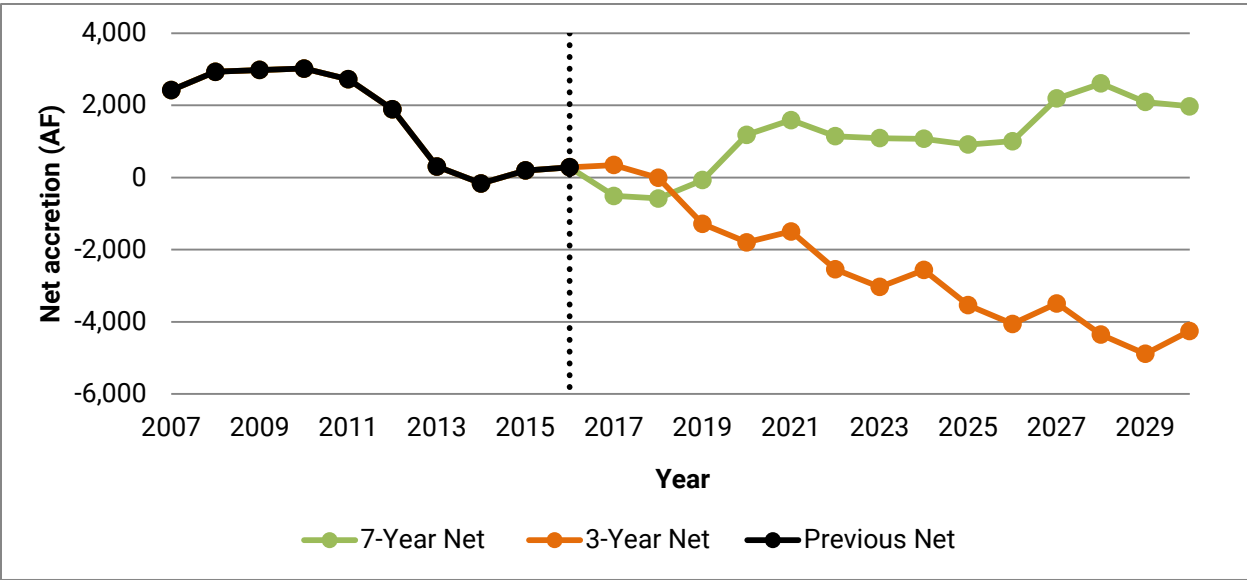
Figure C. 3-Year and 7-Year Net accretion (AF) at the TBNRD Southern Boundary. The 3-year and 7-year projections are described in the captions for Figure A and Figure B.
