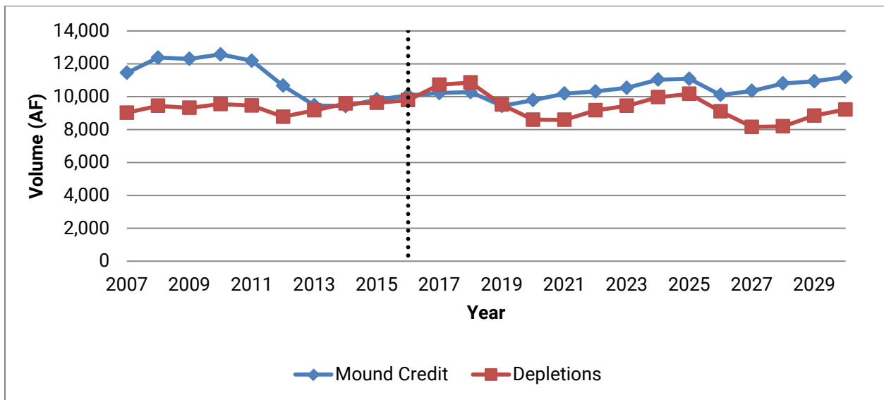
Figure B. 7-Year Mound Credit and Groundwater Depletions (AF) at the TBNRD Southern Boundary. Data from 2010-2016 were projected forward from 2016 to represent a potential outcome under a cycle with more climate variation.
