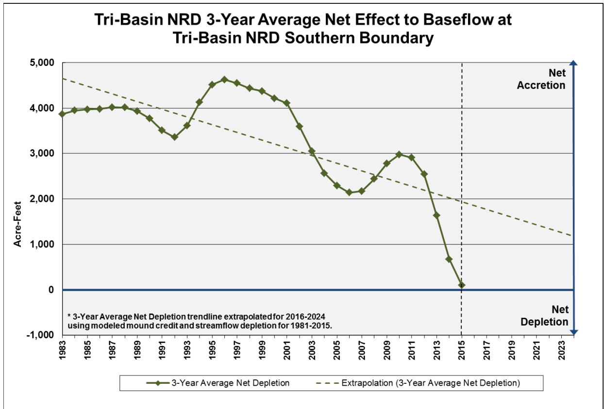
Figure 2: Rolling three-year average net effect to baseflow with trendline.
