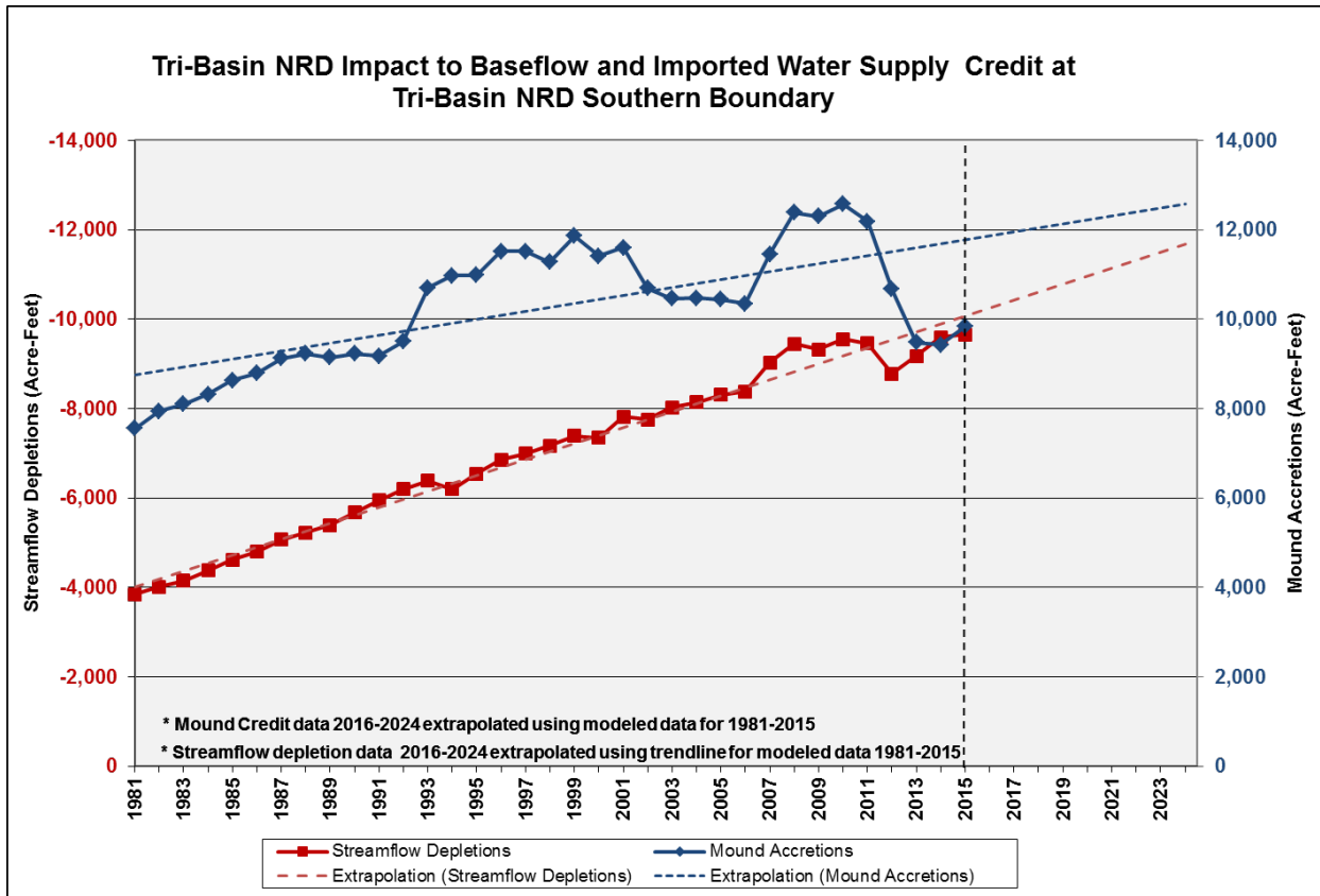
Figure 1: Annual streamflow depletions and mound accretion with trendlines. The data in this figure were calculated using the August 2015 RRCA accounting procedures. In order to show both streamflow depletions and mound accretions for comparison in one chart, the negative values on the left vertical axis pertain to the red line, representing stream depletion values, and positive values on the right vertical axis pertain to the blue line, representing mound accretions.
