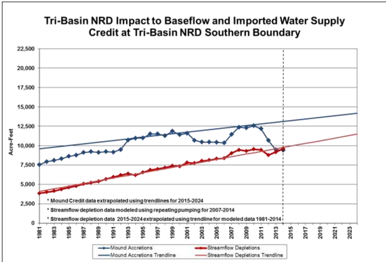
Figure 2: Streamflow depletions and mound accretions data and trendlines. This chart was developed using the “New” RRCA accounting procedures.
