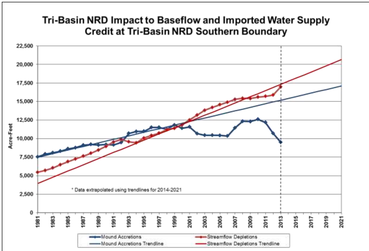
Figure 1: Streamflow depletions and mound accretion data and trendlines. This chart was developed using the “Old” RRCA accounting procedures.
