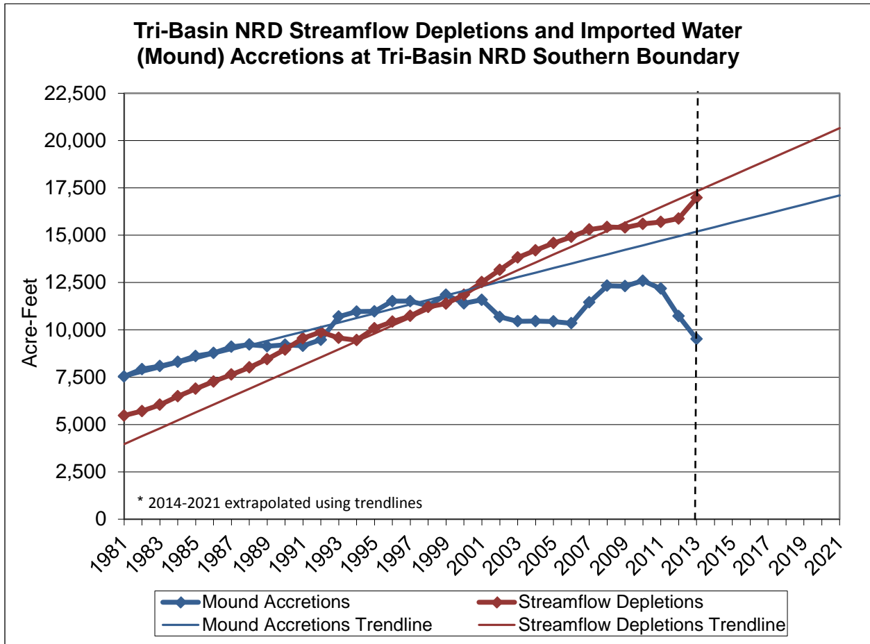
Figure 1. Streamflow depletions and mound accretions data and trendlines. This chart was developed using the current RRCA accounting procedures.
