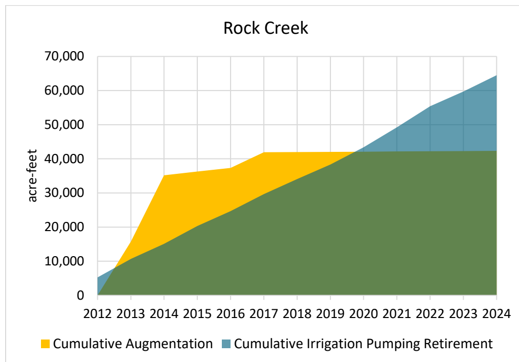
Figure 4: Cumulative water use for augmentation and estimated irrigation pumping on acres purchased under the Rock Creek Augmentation Project.
