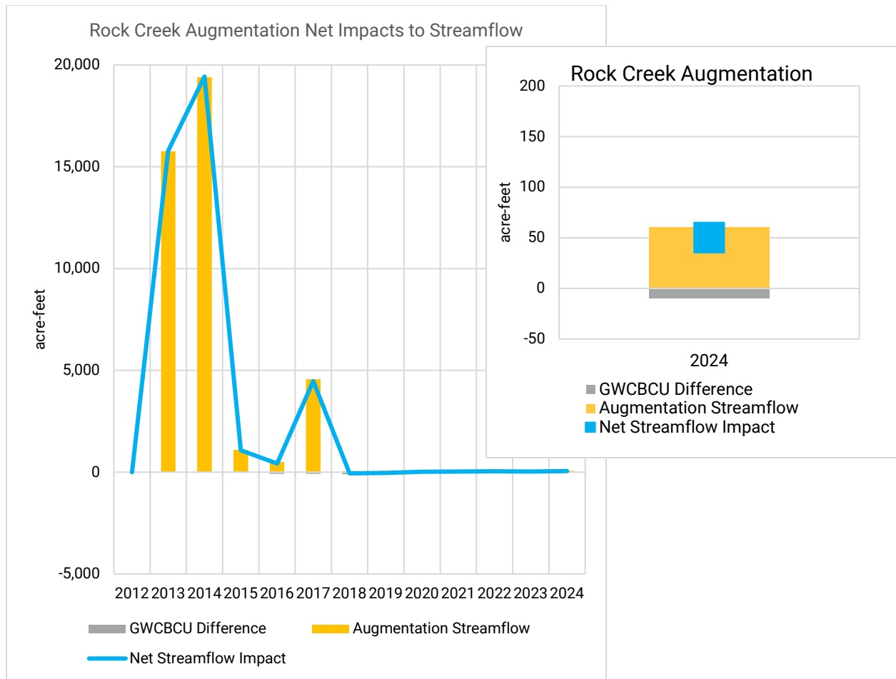
Figure 6: The net impacts to streamflow from the Rock Creek Augmentation Project. 2024 data are final as of this report. An inset is included to show a closeup of 2024. In this figure, a positive value indicates a net increase in streamflow due to Rock Creek project operations, and a negative value indicates net depletions to streamflow. Because of this, the GWCBCU Difference values in this chart are represented as the inverse of the GWCBCU values in Figure 5. The Net Streamflow Impact is the sum of GWCBCU Difference and Augmentation Streamflow.
