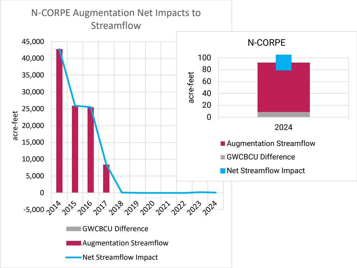
Figure 3: The net impacts to streamflow from the N-CORPE Augmentation Project. 2024 data are final as of this report. An inset is included to show a closeup of 2024. In this figure, a positive value indicates a net increase in streamflow due to N-CORPE operations, and a negative value indicates net depletions to streamflow. Because of this, the GWBCU Difference values in this chart are represented as the inverse of the GWBCU values in Figure 2. The Net Streamflow Impact is the sum of GWBCU Difference and Augmentation Streamflow.
