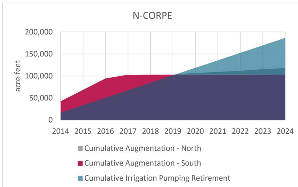
Figure 1: Cumulative water use for augmentation and estimated irrigation pumping on acres purchased under the N-CORPE Augmentation Project.
