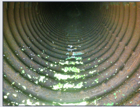
Severely corroded principal spillway pipe in Jefferson County.
